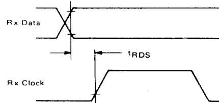
FIGURE 4 — RECEIVE DATA SETUP TIME (+1 Mode)
