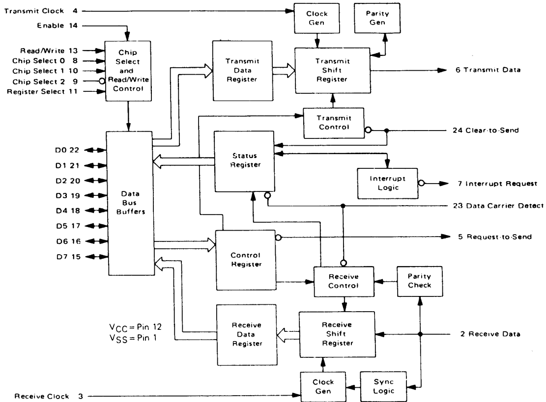
FIGURE 9 — EXPANDED BLOCK DIAGRAM
