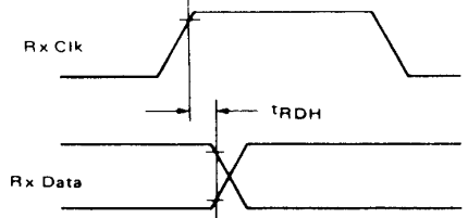
FIGURE 5 — RECEIVE DATA HOLD TIME (+1 Mode)
