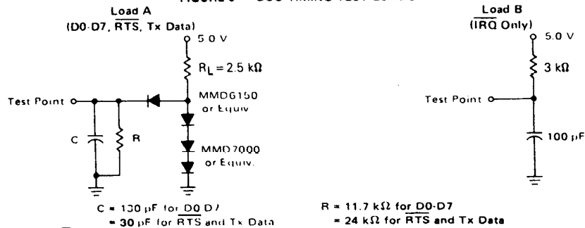
FIGURE 8 — BUS TIMING TEST LOADS
