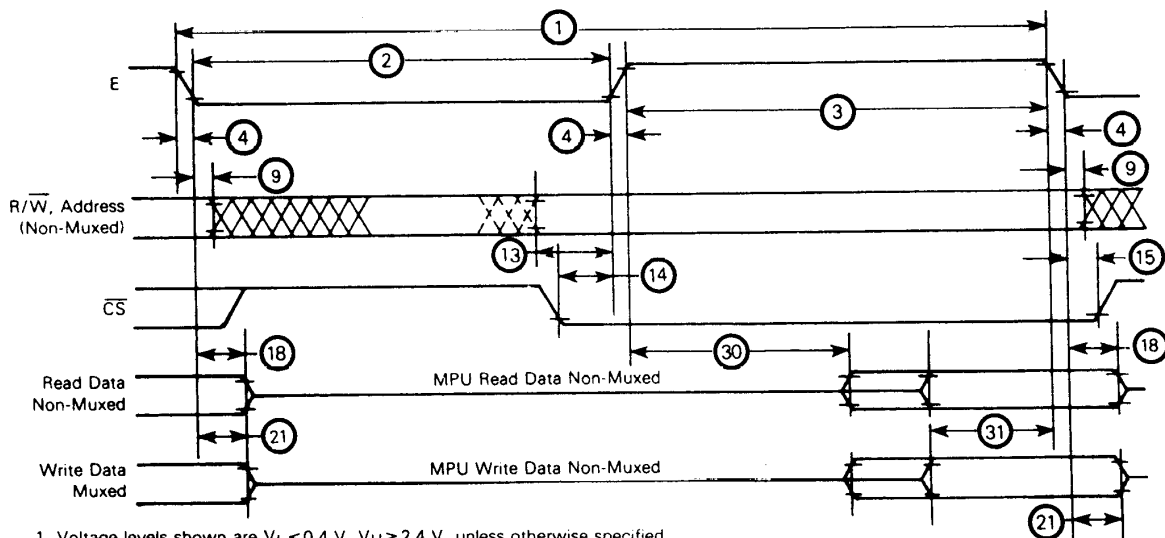
FIGURE 7 — BUS TIMING CHARACTERISTICS
